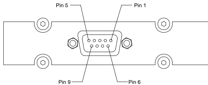
Figure 1: RS 232 Connector Panel 9pin D-Sub female
