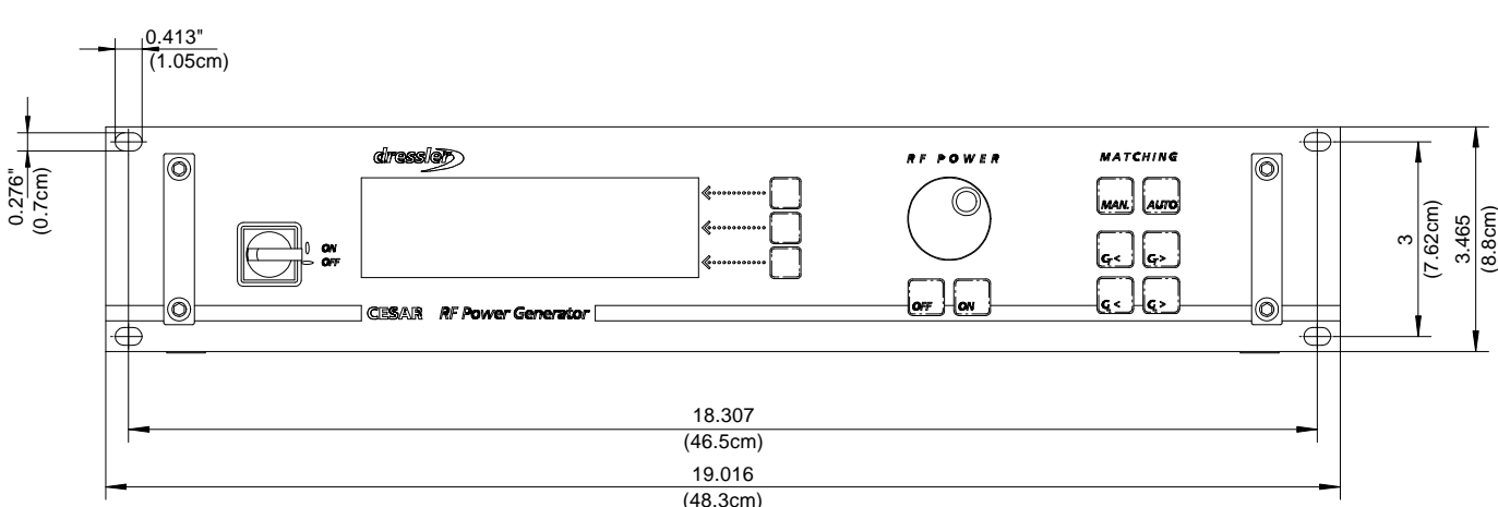
Front view
