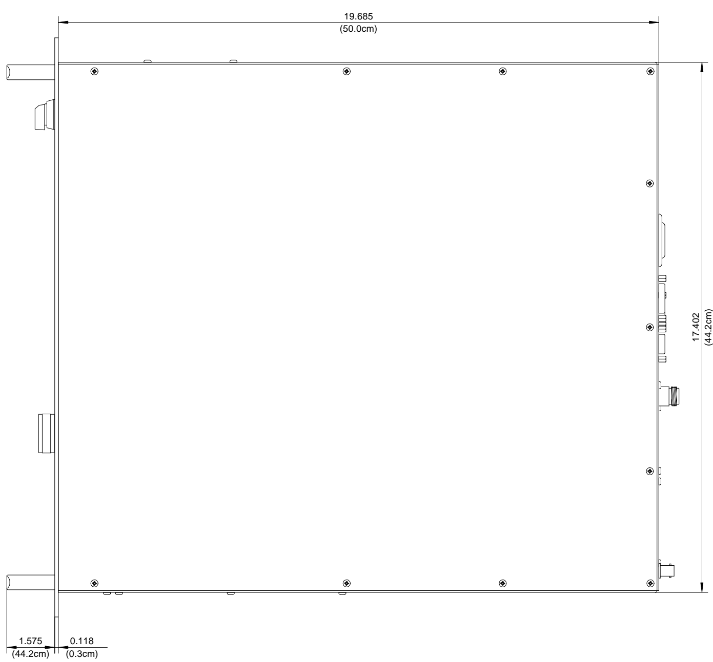
Top view
