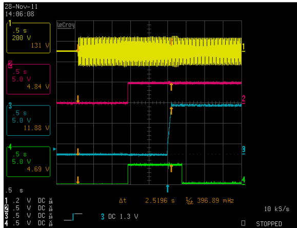
Figure 1: LCM600L Turn-on Delay via AC Mains - Vin = 90Vac Load: Io = 50A (12V), I SB = 2A (5V) Ch 1: AC Mains Ch 2: V SB Ch 3: Vo Ch 4: POWER GOOD
