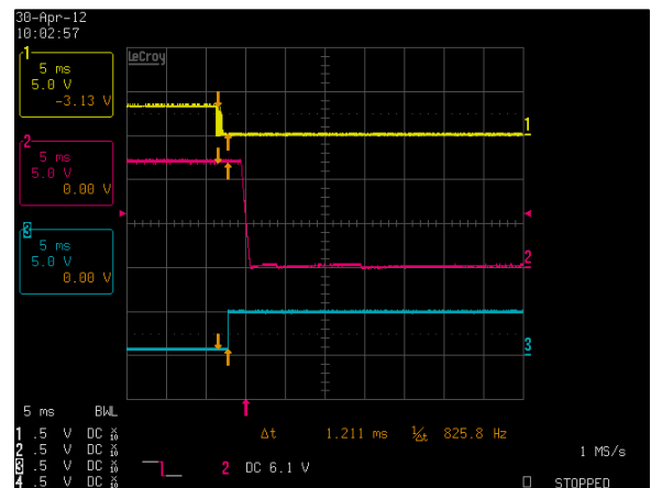
Figure 6: LCM600L Turn-off Characteristic via INH_EN Full Load: Io = 50A (12V), I SB = 2A (5V) Ch 1: INH_EN Ch 2: Vo Ch 3: POWER GOOD
