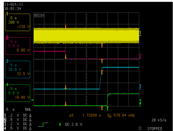
Figure 47: LCM600U Turn-on delay via INH_EN - V_{in} = 90\text{Vac} Full Load: I_o = 16.7\text{A} (36V), I_{SB} = 2\text{A} (5V) Ch 1: AC Mains Ch 2: INH_EN Ch 3: V_o Ch 4: POWER GOOD
