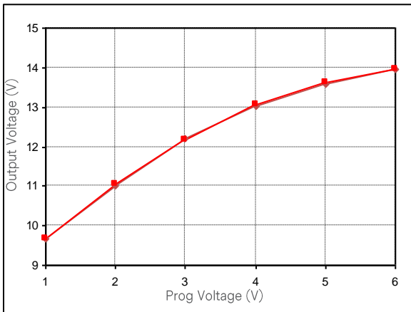
Figure 15: LCM600L Output Voltage Adjustment by Vprog @ 25 degC Loading: I o = 0A (12V), I SB = 0A (5V)
