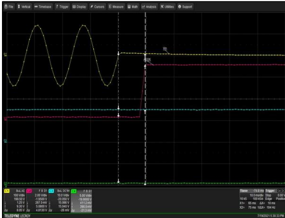
Figure 28: LCM600N ACOK Signal Turn-off Delay - Vin = 100Vac Load: Io = 2A (15V), I SB = 0A (5V) Ch 1: AC Mains Ch 2: ACOK Ch 3: Vo Ch 4: DCOK
