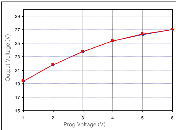
Figure 45: LCM600Q Output Voltage Adjustment by Vprom @ 25 degC Loading: Io = 0A (24V), I SB = 0A (5V)
