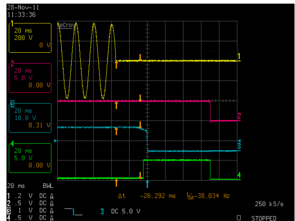
Figure 4: LCM600L Hold-up Time - Vin = 264Vac / 47Hz / 0° Load: Io = 50A (12V), I SB = 2A (5V) Ch 1: AC Mains Ch 2: V SB Ch 3: Vo Ch 4: POWER GOOD
