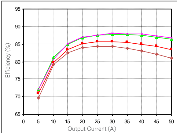
Figure 9: LCM600L Efficiency Curves @ 25 degC, ◆ 90 Vac ■ 115 Vac ▲ 230 Vac ✖ 264 Vac Loading: Vo = 10% increment to 50A, I SB = 0A (5V)
