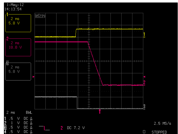
Figure 51: LCM600U Turn-off Characteristic via INH_EN Full Load: I_o = 16.7\text{A} (36V), I_{SB} = 2\text{A} (5V) Ch 1: INH_EN Ch 2: V_o Ch 3: POWER GOOD
