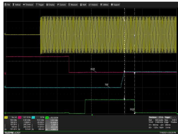
Figure 12: LCM600L DCOK Signal Turn-on Delay - Vin = 100Vac Load: Io = 2A (12V), I SB = 0A (5V) Ch 1: AC Mains Ch 2: ACOK Ch 3: Vo Ch 4: DCOK
