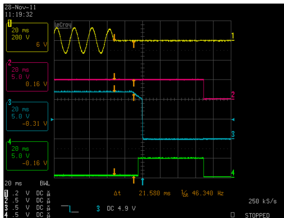
Figure 3: LCM600L Hold-up Time - Vin = 90Vac / 63Hz / 0° Load: Io = 50A (12V), I SB = 2A (5V) Ch 1: AC Mains Ch 2: V SB Ch 3: Vo Ch 4: POWER GOOD
