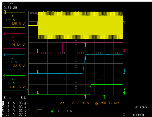
Figure 46: LCM600U Turn-on delay via AC mains - V_{in} = 90\text{Vac} Full Load: I_o = 16.7\text{A} (36V), I_{SB} = 2\text{A} (5V) Ch 1: AC Mains Ch 2: V_{SB} Ch 3: V_o Ch 4: POWER GOOD
