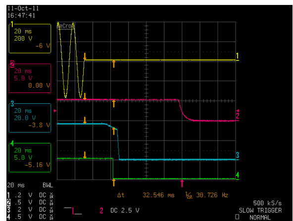
Figure 49: LCM600U Hold-up Time - V_{in} = 264\text{Vac} / 47\text{Hz} / 0^\circ Full Load: I_o = 16.7\text{A} (36V), I_{SB} = 2\text{A} (5V) Ch 1: AC Mains Ch 2: V_{SB} Ch 3: V_o Ch 4: POWER GOOD
