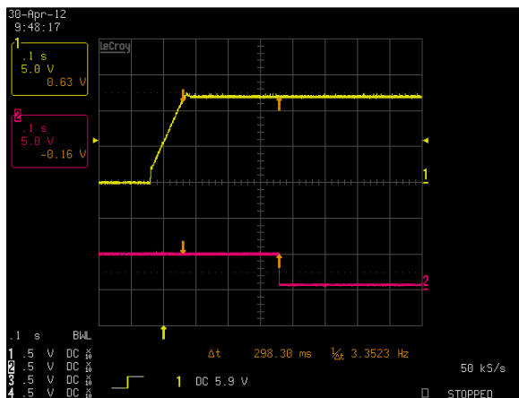
Figure 5: LCM600L Output Voltage Startup Characteristic Vin = 90Vac Full Load: Io = 50A (12V), I SB = 2A (5V) Ch 1: Vo Ch 2: POWER GOOD
