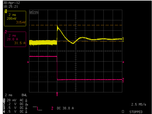
Figure 8: LCM600L Transient Response - Vo Deviation (high to low) 100% to 10% load change 1A/uS slew rate Vin = 230Vac Ch 1: Vo Ch 2: Io
