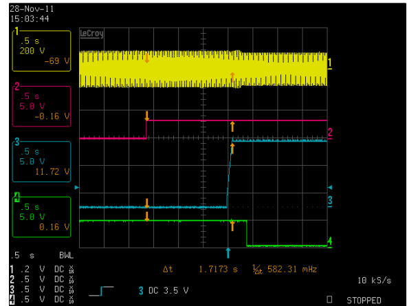
Figure 2: LCM600L Turn-on Delay via INH_EN - Vin = 90Vac Load: Io = 50A (12V), I SB = 2A (5V) Ch 1: AC Mains Ch 2: V SB Ch 3: Vo Ch 4: POWER GOOD
