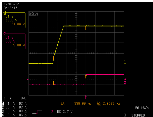
Figure 50: LCM600U Output Voltage Startup Characteristic V_{in} = 90\text{Vac} Full Load: I_o = 16.7\text{A} (36V), I_{SB} = 2\text{A} (5V) Ch 1: V_o Ch 2: POWER GOOD
