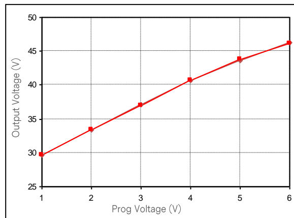
Figure 56: LCM600U Output Voltage Adjustment by Vprom @ 25 degC ◆ 115 Vac ■ 230 Vac Loading: Io = 0A (36V), I SB = 0A (5V)
