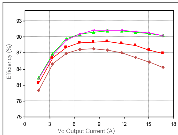
Figure 54: LCM600U Efficiency Curves @ 25 degC ◆ 90 Vac ■ 115 Vac ▲ 230 Vac ◆ 264 Vac Loading: Vo = 10% increment to 16.7A, I SB = 0A (5V)
