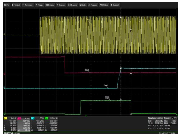
Figure 27: LCM600N ACOK Signal Turn-on Delay - Vin = 100Vac Load: Io = 2A (15V), I SB = 0A (5V) Ch 1: AC Mains Ch 2: ACOK Ch 3: Vo Ch 4: DCOK
