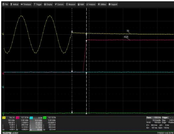
Figure 13: LCM600L ACOK Signal Turn-off Delay - Vin = 100Vac Load: Io = 2A (12V), I SB = 0A (5V) Ch 1: AC Mains Ch 2: ACOK Ch 3: Vo Ch 4: DCOK
