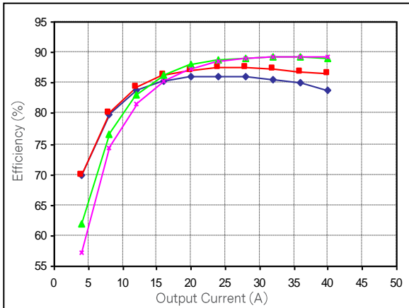
Figure 24: LCM600N Efficiency Curves @ 25 degC ◆ 90 Vac ■ 115 Vac ▲ 230 Vac ★ 264 Vac Loading: Vo = 10% increment to 40A, I SB = 0A (5V)
