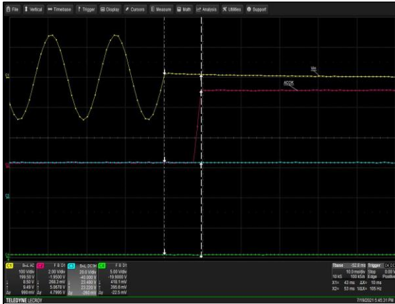
Figure 43: LCM600Q ACOK Signal Turn-off Delay - Vin = 100Vac Load: Io = 2A (24V), I SB = 0A (5V) Ch 1: AC Mains Ch 2: ACOK Ch 3: Vo Ch 4: DCOK
