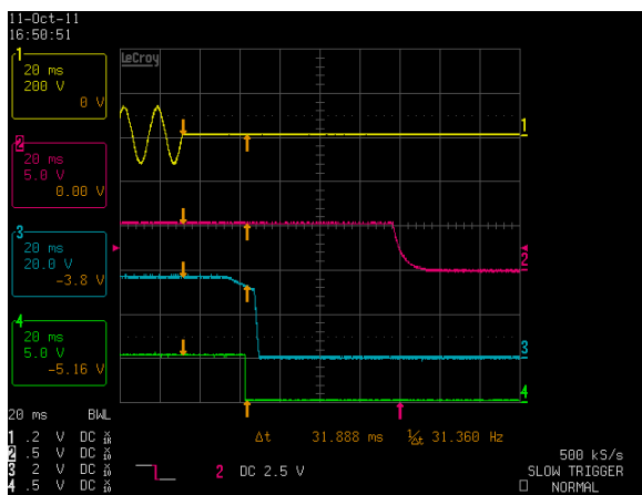
Figure 48: LCM600U Hold-up Time - V_{in} = 90\text{Vac} / 63\text{Hz} / 0^\circ Full Load: I_o = 16.7\text{A} (36V), I_{SB} = 2\text{A} (5V) Ch 1: AC Mains Ch 2: V_{SB} Ch 3: V_o Ch 4: POWER GOOD
