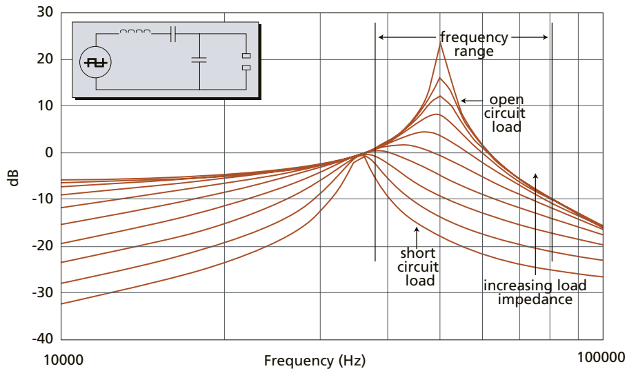
Figure 1 LCC topology with gain curves
