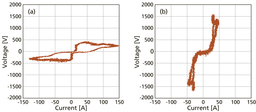
Figure 2 Measured V/I plots for a) reactive and b) metallic Al DMS process
