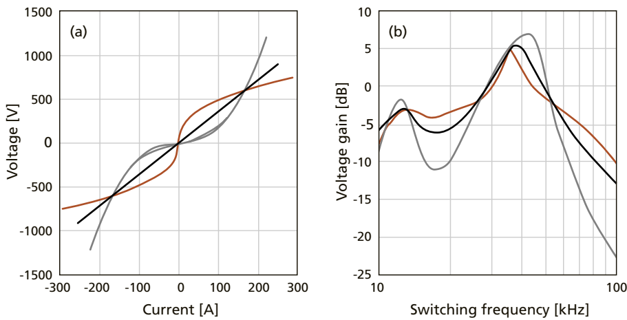
Figure 3 a) Load characteristics and b) gain curves for each respective load
