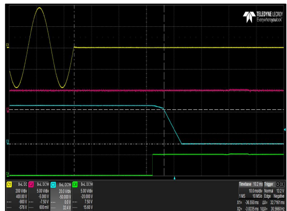
Figure 37: LCM300U Hold-up Time Vin = 264Vac / 60Hz / 0° Load: Io = 8.4A (36V), I SB = 2A (5V) Ch 1: AC Mains Ch 2: V SB Ch 3: Vo Ch 4: G_DCOK_C
