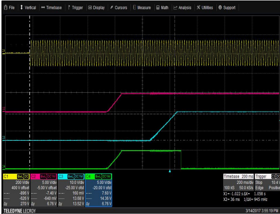
Figure 12: LCM300N Turn-on delay via AC mains Vin = 90Vac Load: I O = 20A (15V), I SB = 2A (5V) Ch 1: AC Mains Ch 2: V SB Ch 3: V O Ch 4: G_DCOK_C
