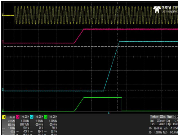
Figure 34: LCM300U Turn-on delay via AC mains Vin = 90Vac Load: Io = 8.4A (36V), I SB = 2A (5V) Ch 1: AC Mains Ch 2: V SB Ch 3: Vo Ch 4: G_DCOK_C
