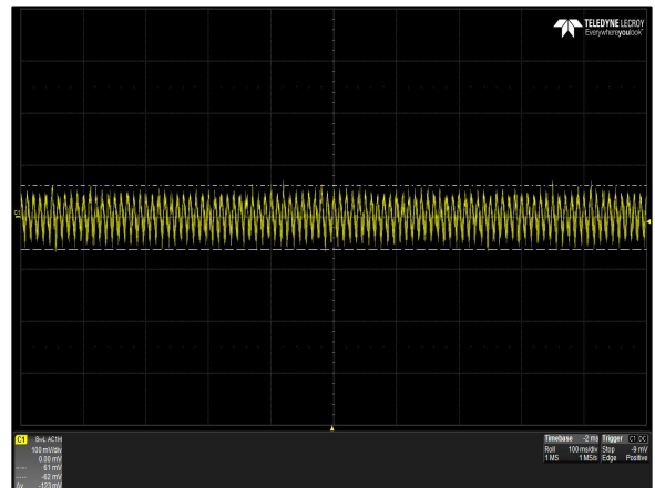
Figure 43: LCM300U Ripple and Noise Measurement Vin = 90Vac Load: Io = 8.4A (36V), I_{SB} = 2A (5V) Ch 1: Vo
