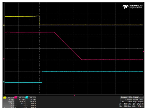
Figure 50: LCM300W Turn Off Characteristic via INH_EN Load: Io = 6.3A (48V), I SB = 2A (5V) Ch 1: INH_EN Ch 2: Vo Ch 3: G_DCOK_C
