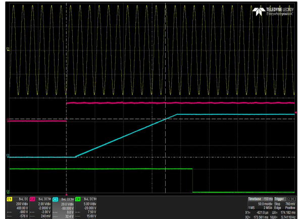
Figure 35: LCM300U Turn-on delay via INH_EN Vin = 90Vac Load: Io = 8.4A (36V), I SB = 2A (5V) Ch 1: AC Mains Ch 2: INH_EN Ch 3: Vo Ch 4: G_DCOK_C
