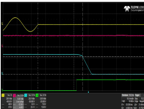
Figure 36: LCM300U Hold-up Time Vin = 90Vac / 47Hz / 0° Load: Io = 8.4A (36V), I SB = 2A (5V) Ch 1: AC Mains Ch 2: V SB Ch 3: Vo Ch 4: G_DCOK_C
