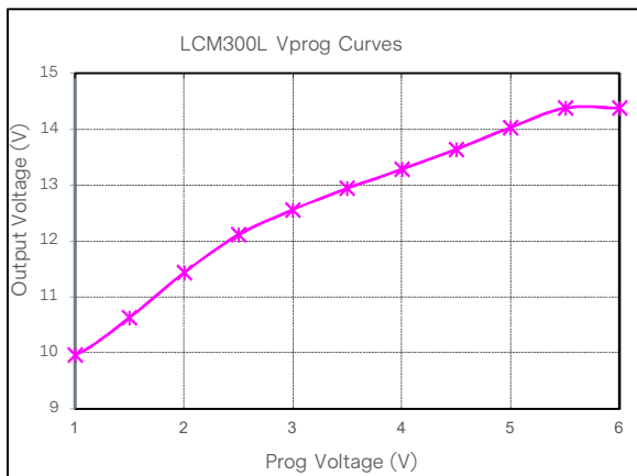
Figure 11: LCM300L Output Voltage Adjustment by Vprog @ 25°C Loading: I_O = 0A (12V), I_{SB} = 0A (5V)
