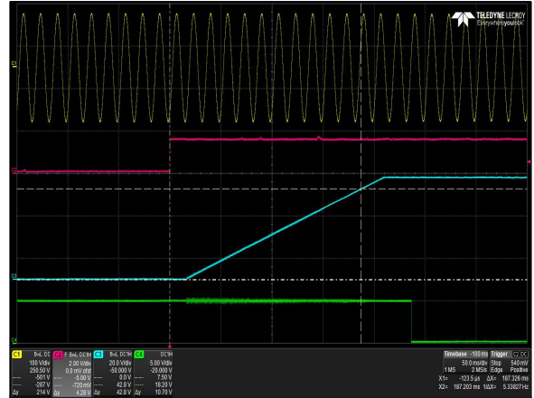
Figure 46: LCM300W Turn-on delay via INH_EN Vin = 90Vac Load: Io = 6.3A (48V), I SB = 2A (5V) Ch 1: AC Mains Ch 2: INH_EN Ch 3: Vo Ch 4: G_DCOK_C
