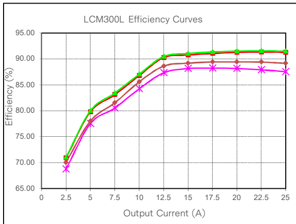
Figure 9: LCM300L Efficiency Curve @ 25°C Loading: I_{o\_main} = 10% I_{o\_max} increment to 25A, I_{SB} = 0A (5V)
