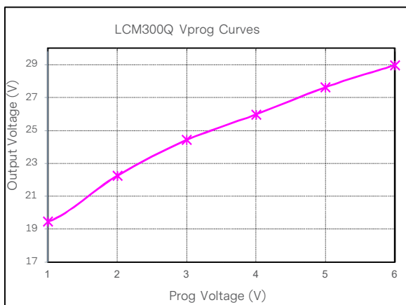
Figure 33: LCM300Q Output Voltage Adjustment by V_{prog} @ 25°C — 115Vac Loading: I_O = 0A (24V), I_{SB} = 0A (5V)
