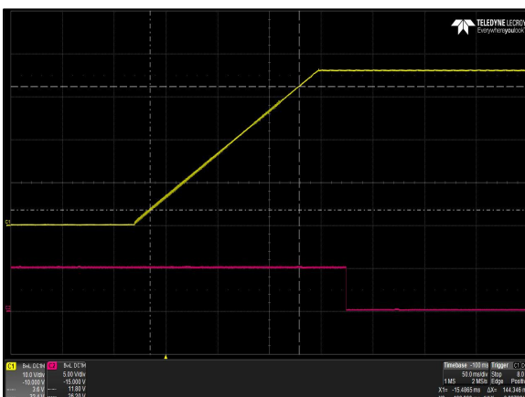
Figure 38: LCM300U Output Voltage Startup Characteristic Vin = 90Vac Load: Io = 8.4A (36V), I SB = 2A (5V) Ch 1: Vo Ch 2: G_DCOK_C
