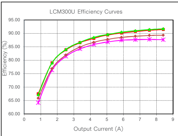
Figure 42: LCM300U Efficiency Curve @ 25°C — 90Vac — 115Vac — 230Vac — 264Vac Loading: I_{o\_main} = 10\%I_{o\_max} increment to 8.4A, I_{SB} = 0A (5V)
