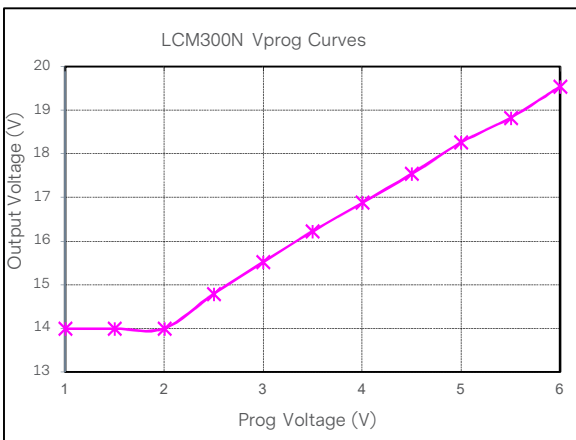
Figure 22: LCM300N Output Voltage Adjustment by Vprog @ 25°C - 115Vac (magenta x) Loading: I_O = 0A (15V), I_{SB} = 0A (5V)
