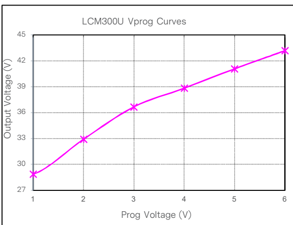
Figure 44: LCM300U Output Voltage Adjustment by Vprog @ 25°C — 115Vac Loading: I_o = 0A (36V), I_{SB} = 0A (5V)
