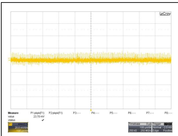
Figure 51: AYA01A12-L Ripple and Noise Measurement Vin = 12Vdc Load: Io = 0.6A Ch 1: Vo
