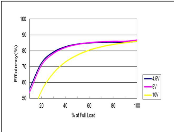
Figure 37: AYA01CC05-L Efficiency Versus Output Current Curve Vin = 4.5 to 10Vdc Load: Io = 0 to ±0.1A
