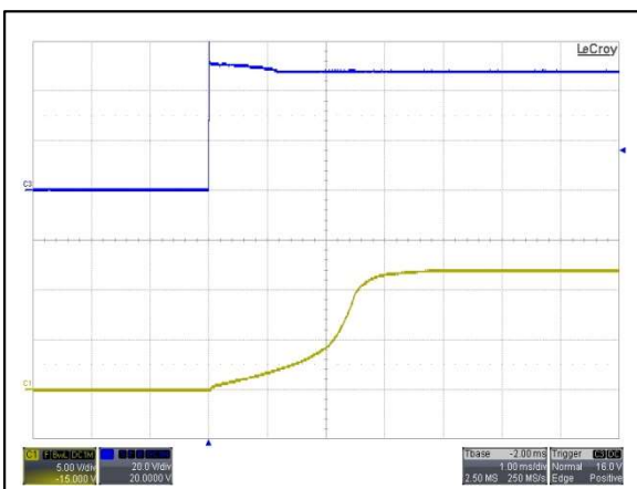
Figure 143: AYA01B48-L Output Voltage Startup Characteristic by Vin Vin = 48Vdc Load: Io = 0.25A Ch 3: Vin Ch 1: Vo
