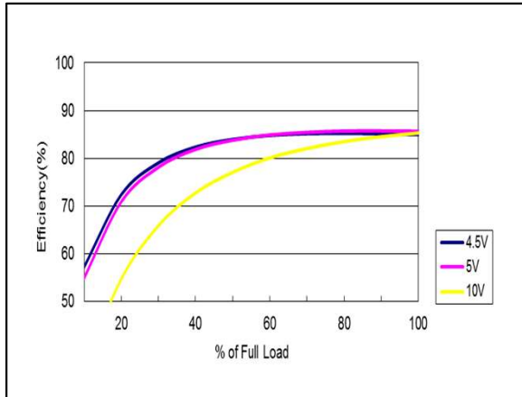
Figure 31: AYA01BB05-L Efficiency Versus Output Current Curve Vin = 4.5 to 10Vdc Load: I_o = 0 to \pm 0.125A
