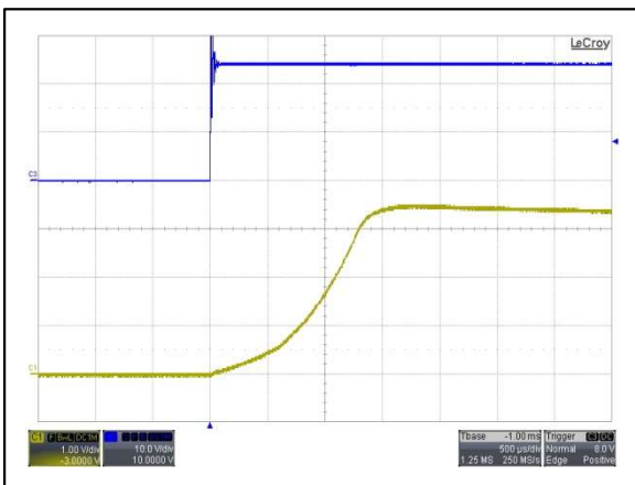
Figure 89: AYA01F24-L Output Voltage Startup Characteristic by Vin Vin = 24Vdc Load: Io = 0.6A Ch 3: Vin Ch 1: Vo
