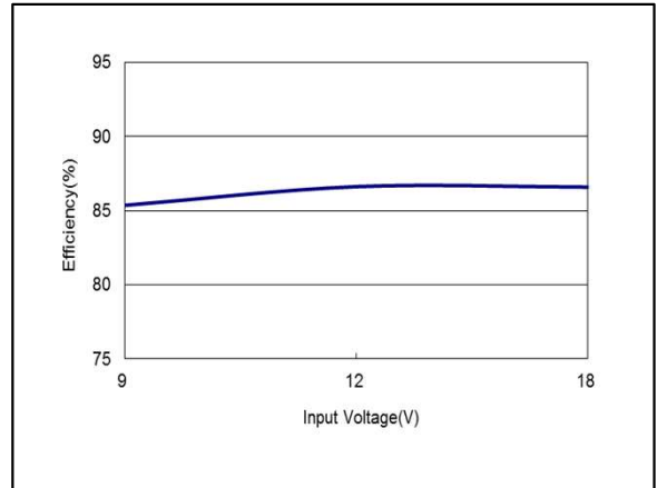
Figure 68: AYA01AA12-L Efficiency Versus Input Voltage Curve Vin = 9 to 18Vdc Load: Io = ±0.3A
