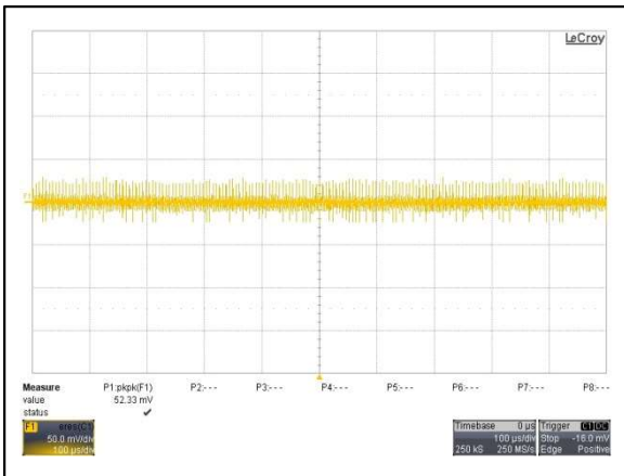
Figure 57: AYA01B12-L Ripple and Noise Measurement Vin = 12Vdc Load: Io = 0.25A Ch 1: Vo
