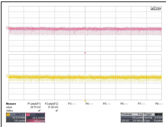
Figure 69: AYA01AA12-L Ripple and Noise Measurement Vin = 12Vdc Load: Io = ±0.3A Ch 1: Vo
