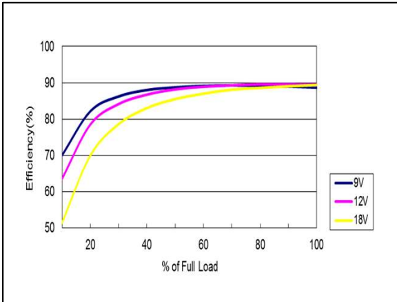
Figure 55: AYA01B12-L Efficiency Versus Output Current Curve Vin = 9 to 18Vdc Load: Io = 0 to 0.25A
