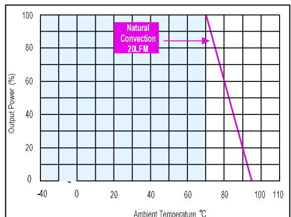
Figure 30: AYA01AA05-L Derating Curve Vin = 5Vdc
