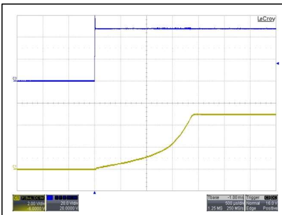
Figure 137: AYA01A48-L Output Voltage Startup Characteristic by Vin Vin = 48Vdc Load: Io = 0.6A Ch 3: Vin Ch 1: Vo
