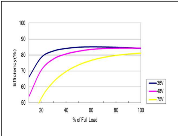
Figure 133: AYA01A48-L Efficiency Versus Output Current Curve Vin = 36 to 75Vdc Load: Io = 0 to 0.6A
