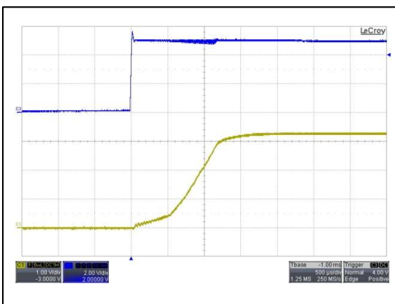
Figure 5: AYA01F05-L Output Voltage Startup Characteristic by Vin Vin = 5Vdc Load: Io = 0.6A Ch 3: Vin Ch 1: Vo
