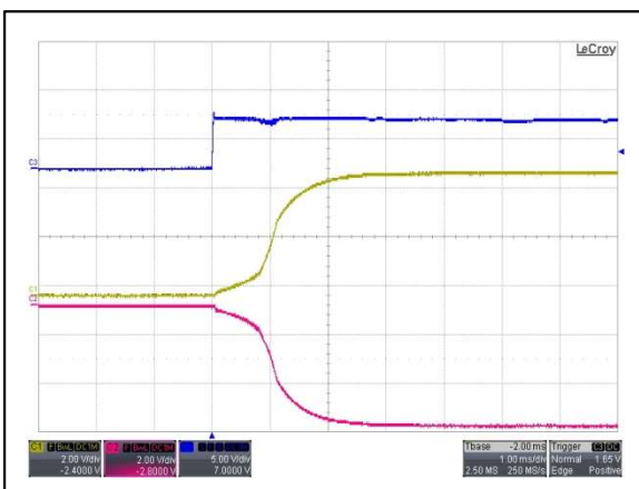
Figure 29: AYA01AA05-L Output Voltage Startup Characteristic by Vin Vin = 5Vdc Load: lo = ±0.3A Ch 3: Vin Ch 1: Vo1 Ch 2: Vo2
