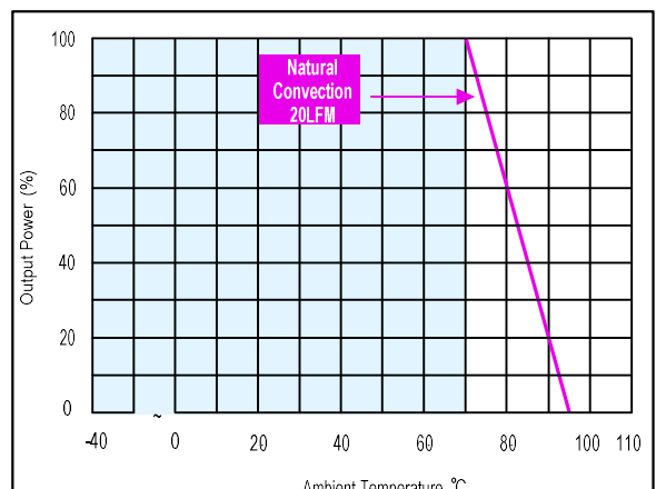
Figure 42: AYA01CC05-L Derating Curve Vin = 5Vdc
