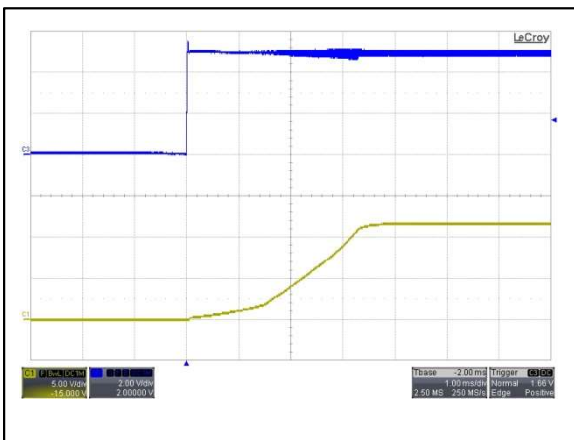
Figure 17: AYA01B05-L Output Voltage Startup Characteristic by Vin Vin = 5Vdc Load: Io = 0.25A Ch 3: Vin Ch 1: Vo
