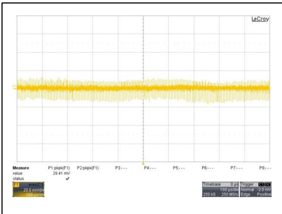
Figure 87: AYA01F24-L Ripple and Noise Measurement Vin = 24Vdc Load: Io = 0.6A Ch 1: Vo
