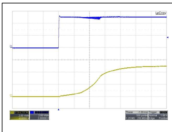
Figure 11: AYA01A05-L Output Voltage Startup Characteristic by Vin Vin = 5Vdc Load: Io = 0.6A Ch 3: Vin Ch 1: Vo
