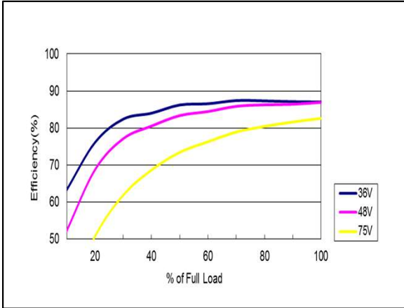
Figure 157: AYA01BB48-L Efficiency Versus Output Current Curve Vin = 36 to 75Vdc Load: I_o = 0 to \pm 0.125A
