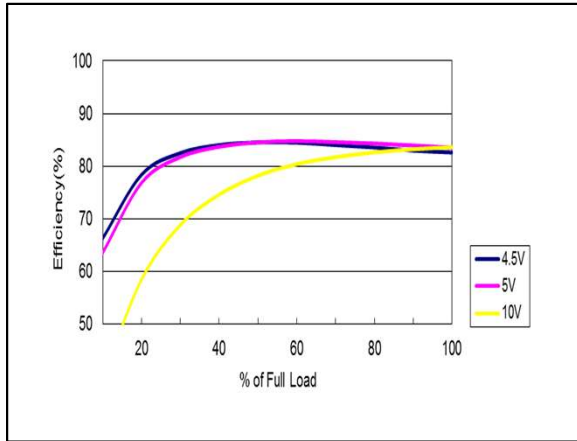
Figure 7: AYA01A05-L Efficiency Versus Output Current Curve Vin = 4.5 to 10Vdc Load: Io = 0 to 0.6A
