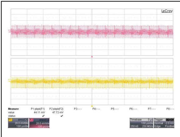
Figure 111: AYA01AA24-L Ripple and Noise Measurement Vin = 24Vdc Load: Io = ±0.3A Ch 1: Vo1 Ch 2: Vo2
