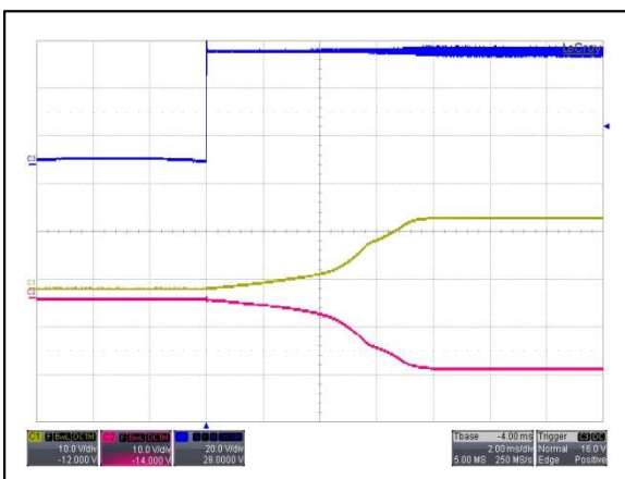
Figure 167: AYA01CC48-L Output Voltage Startup Characteristic by Vin Vin = 48Vdc Load: I_o = \pm 0.1A Ch 3: Vin Ch 1: Vo1 Ch 2: Vo2
