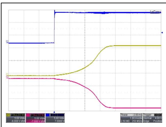
Figure 77: AYA01BB12-L Output Voltage Startup Characteristic by Vin Vin = 12Vdc Load: Io = ±0.1A Ch 3: Vin Ch 1: Vo1 Ch 2: Vo2
