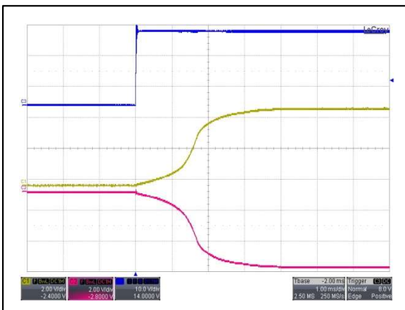
Figure 113: AYA01AA24-L Output Voltage Startup Characteristic by Vin Vin = 24Vdc Load: Io = ±0.3A Ch 3: Vin Ch 1: Vo1 Ch 2: Vo2
