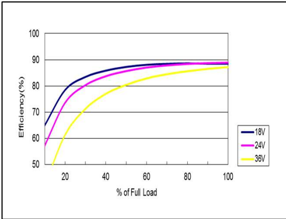
Figure 121: AYA01CC24-L Efficiency Versus Output Current Curve Vin = 18 to 36Vdc Load: Io = 0 to ±0.1A
