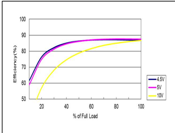
Figure 19: AYA01C05-L Efficiency Versus Output Current Curve Vin = 4.5 to 10Vdc Load: Io = 0 to 0.2A
