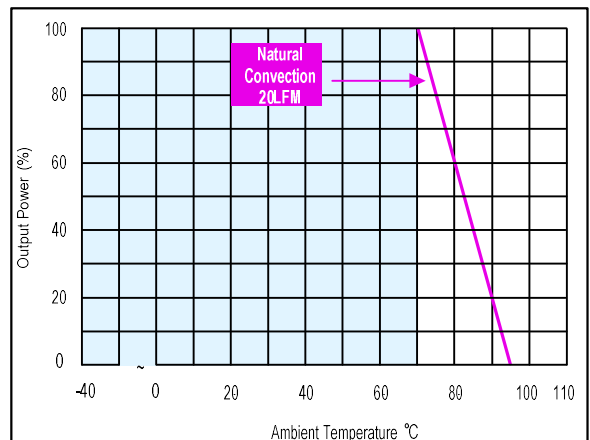
Figure 18: AYA01B05-L Derating Curve Vin = 5Vdc
