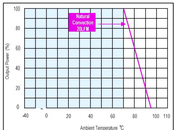
Figure 84: AYA01CC12-L Derating Curve Vin = 12Vdc
