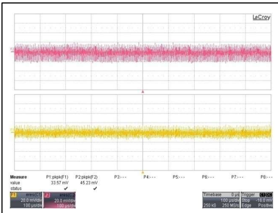
Figure 165: AYA01CC48-L Ripple and Noise Measurement Vin = 48Vdc Load: I_o = \pm 0.1A Ch 1: Vo
