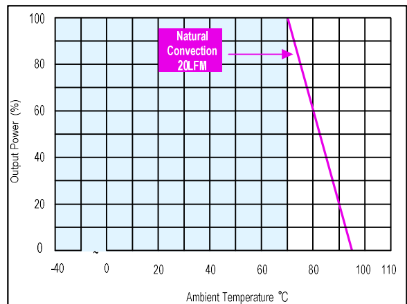
Figure 114: AYA01AA24-L Derating Curve Vin = 24Vdc
