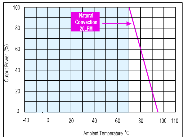
Figure 162: AYA01BB48-L Derating Curve Vin = 48Vdc
