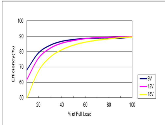
Figure 79: AYA01CC12-L Efficiency Versus Output Current Curve Vin = 9 to 18Vdc Load: Io = 0 to ±0.1A
