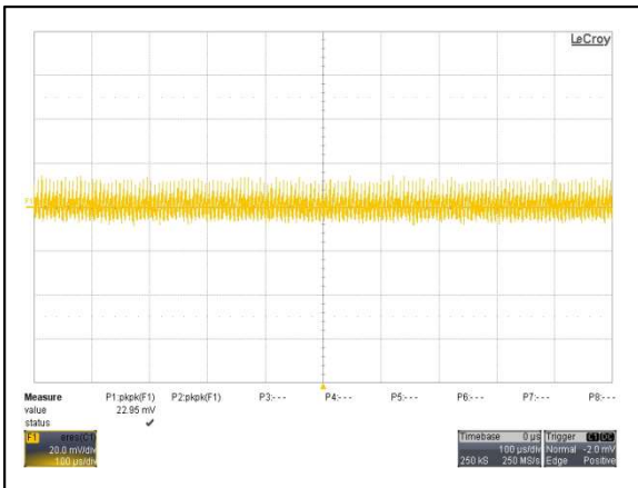
Figure 15: AYA01B05-L Ripple and Noise Measurement Vin = 5Vdc Load: Io = 0.25A Ch 1: Vo
