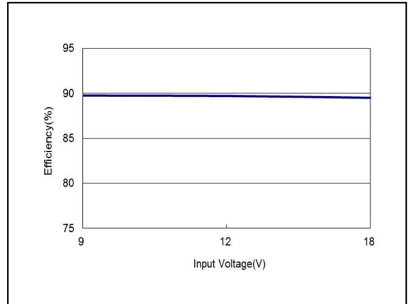
Figure 80: AYA01CC12-L Efficiency Versus Input Voltage Curve Vin = 9 to 18Vdc Load: Io = ±0.1A
