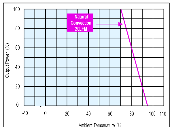
Figure 54: AYA01A12-L Derating Curve Vin = 12Vdc
