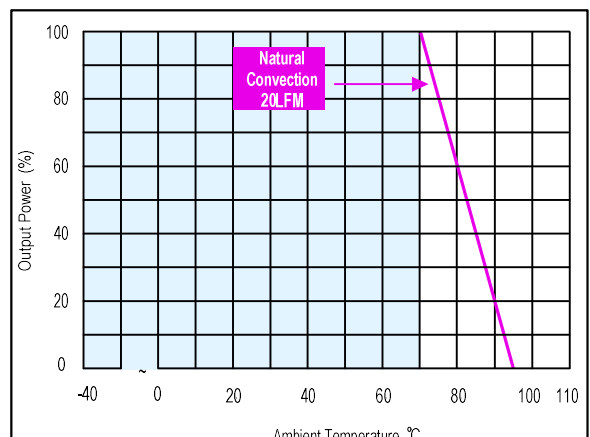
Figure 108: AYA01C24-L Derating Curve Vin = 24Vdc
