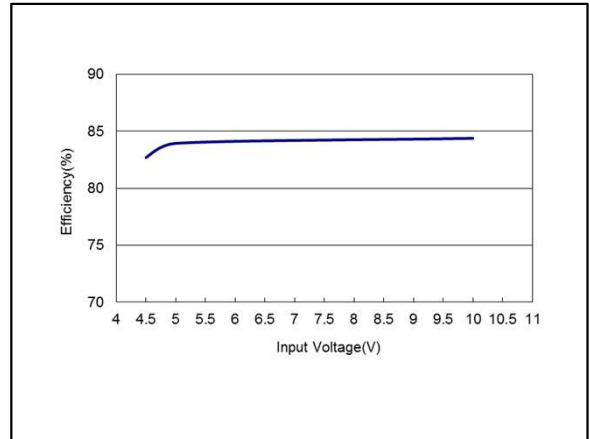
Figure 26: AYA01AA05-L Efficiency Versus Input Voltage Curve Vin = 4.5 to 10Vdc Load: lo = ±0.3A
