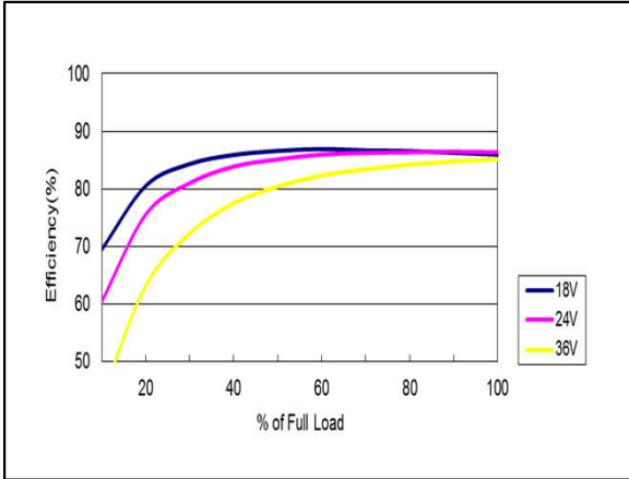
Figure 109: AYA01AA24-L Efficiency Versus Output Current Curve Vin = 18 to 36Vdc Load: Io = 0 to ±0.3A
