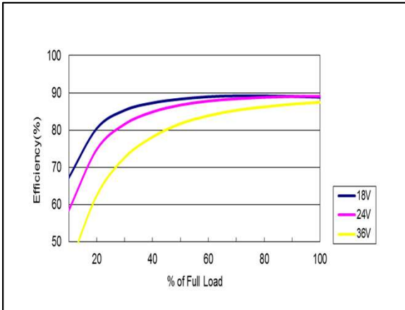
Figure 97: AYA01B24-L Efficiency Versus Output Current Curve Vin = 18 to 36Vdc Load: Io = 0 to 0.25A
