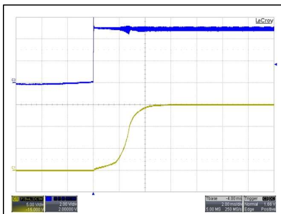
Figure 23: AYA01C05-L Output Voltage Startup Characteristic by Vin Vin = 5Vdc Load: Io = 0.2A Ch 3: Vin Ch 1: Vo
