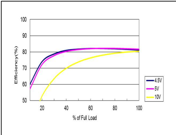
Figure 1: AYA01F05-L Efficiency Versus Output Current Curve Vin = 4.5 to 10Vdc Load: Io = 0 to 0.6A
