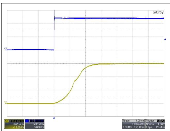
Figure 65: AYA01C12-L Output Voltage Startup Characteristic by Vin Vin = 12Vdc Load: Io = 0.2A Ch 3: Vin Ch 1: Vo
