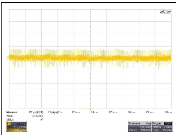
Figure 63: AYA01C12-L Ripple and Noise Measurement Vin = 12Vdc Load: Io = 0.2A Ch 1: Vo
