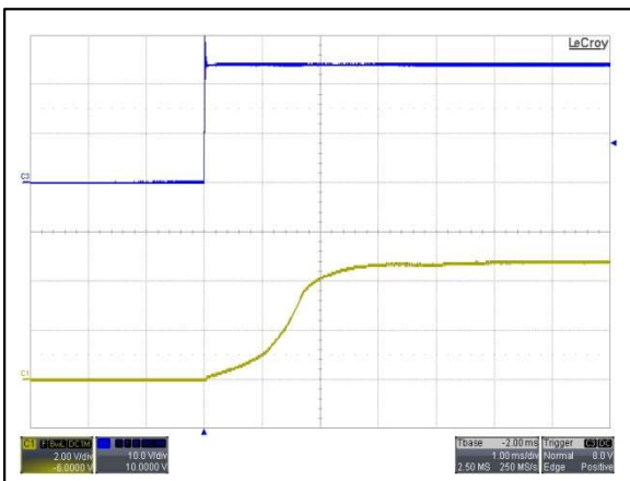
Figure 95: AYA01A24-L Output Voltage Startup Characteristic by Vin Vin = 24Vdc Load: Io = 0.6A Ch 3: Vin Ch 1: Vo
