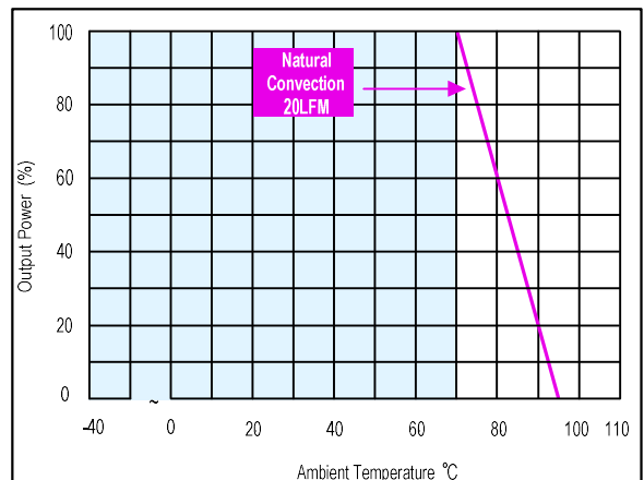
Figure 150: AYA01C48-L Derating Curve Vin = 48Vdc
