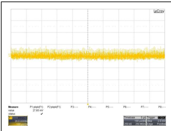
Figure 99: AYA01B24-L Ripple and Noise Measurement Vin = 24Vdc Load: Io = 0.25A Ch 1: Vo
