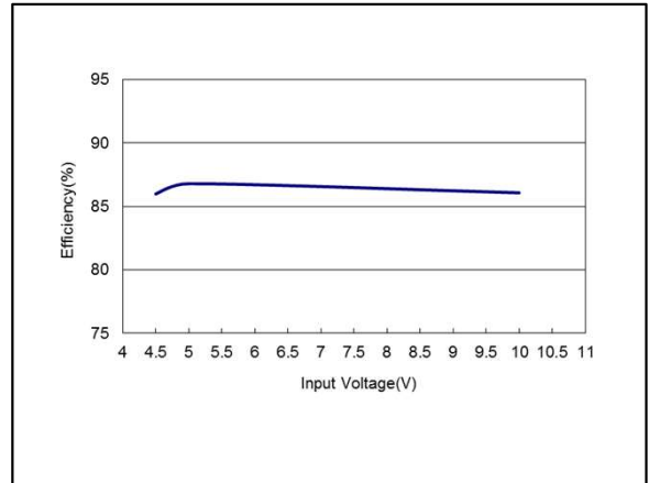
Figure 38: AYA01CC05-L Efficiency Versus Input Voltage Curve Vin = 4.5 to 10Vdc Load: Io = ±0.1A
