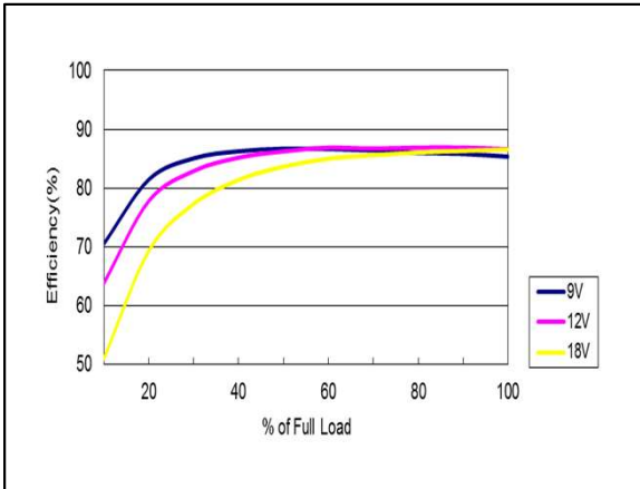
Figure 67: AYA01AA12-L Efficiency Versus Output Current Curve Vin = 9 to 18Vdc Load: Io = 0 to ±0.3A
