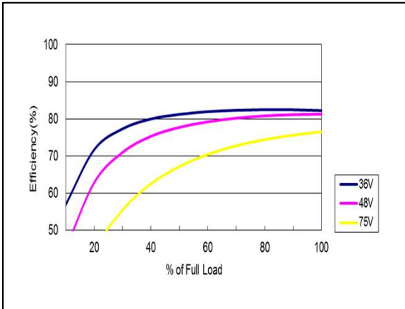
Figure 127: AYA01F48-L Efficiency Versus Output Current Curve Vin = 36 to 75Vdc Load: Io = 0 to 0.6A
