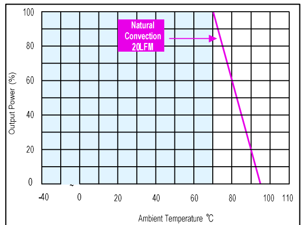
Figure 60: AYA01B12-L Derating Curve Vin = 12Vdc
