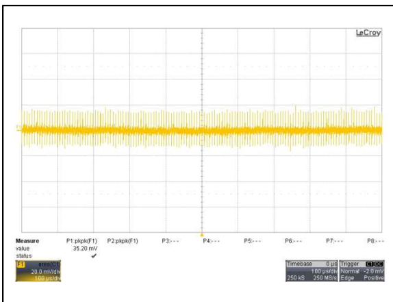
Figure 3: AYA01F05-L Ripple and Noise Measurement Vin = 5Vdc Load: Io = 0.6A Ch 1: Vo
