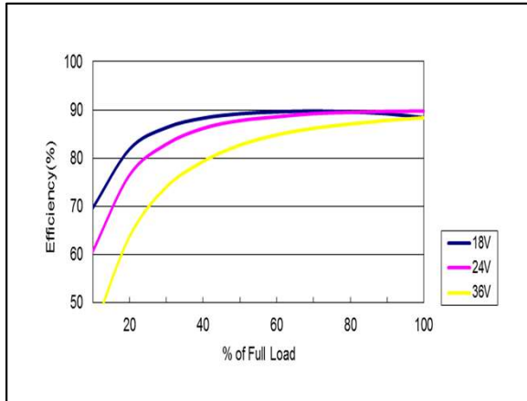
Figure 103: AYA01C24-L Efficiency Versus Output Current Curve Vin = 18 to 36Vdc Load: Io = 0 to 0.2A
