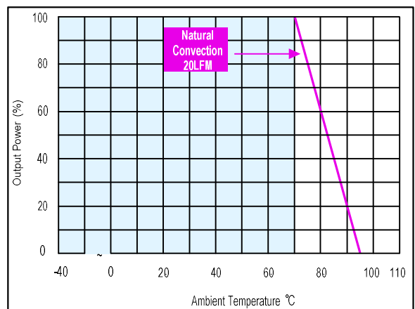
Figure 78: AYA01BB12-L Derating Curve Vin = 12Vdc
