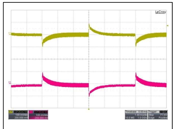
Figure 28: AYA01AA05-L Transient Response Vin = 5Vdc Load: lo = 100% to 75% load change Ch 1: Vo1 Ch 2: Vo2
