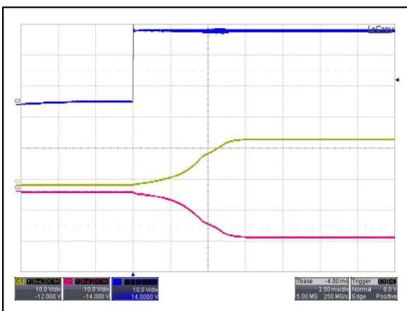
Figure 125: AYA01CC24-L Output Voltage Startup Characteristic by Vin Vin = 24Vdc Load: Io = ±0.1A Ch 3: Vin Ch 1: Vo1 Ch 2: Vo2
