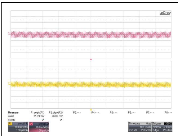
Figure 27: AYA01AA05-L Ripple and Noise Measurement Vin = 5Vdc Load: lo = ±0.3A Ch 1: Vo1 Ch 2: Vo2
