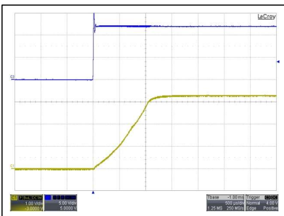
Figure 47: AYA01F12-L Output Voltage Startup Characteristic by Vin Vin = 12Vdc Load: Io = 0.6A Ch 3: Vin Ch 1: Vo
