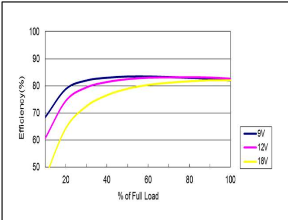
Figure 43: AYA01F12-L Efficiency Versus Output Current Curve Vin = 9 to 18Vdc Load: Io = 0 to 0.6A
