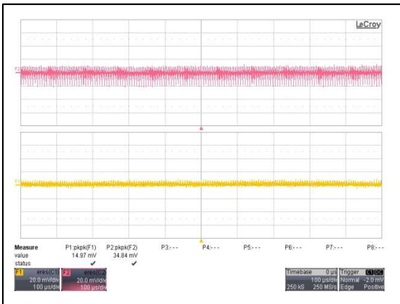
Figure 123: AYA01CC24-L Ripple and Noise Measurement Vin = 24Vdc Load: Io = ±0.1A Ch 1: Vo1 Ch 2: Vo2
