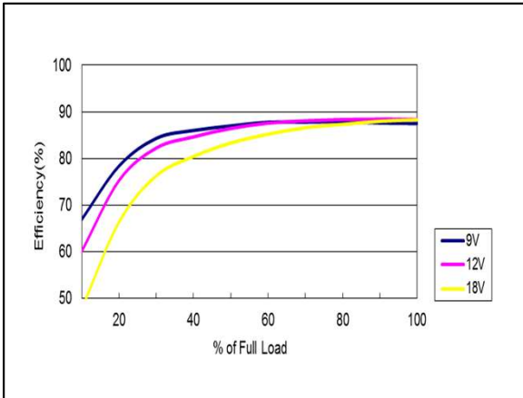
Figure 73: AYA01BB12-L Efficiency Versus Output Current Curve Vin = 9 to 18Vdc Load: Io = 0 to ±0.1A
