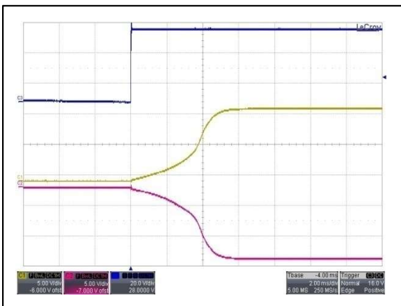
Figure 161: AYA01BB48-L Output Voltage Startup Characteristic by Vin Vin = 48Vdc Load: I_o = \pm 0.125A Ch 3: Vin Ch 1: Vo1 Ch 2: Vo2
