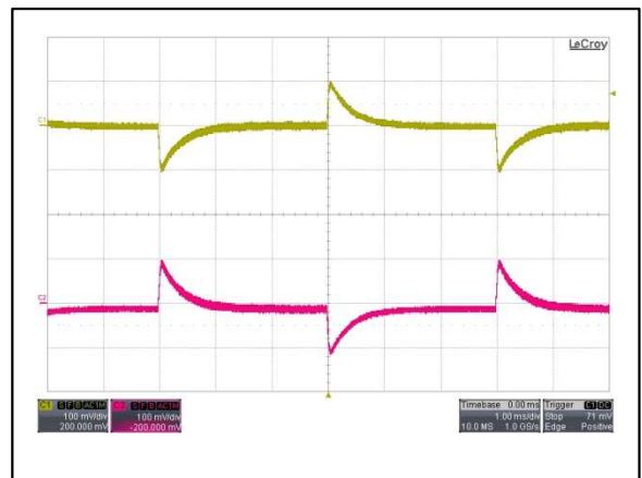
Figure 40: AYA01CC05-L Transient Response Vin = 5Vdc Load: Io = 100% to 75% load change Ch 1: Vo1 Ch 2: Vo2
