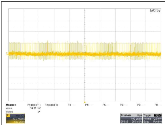
Figure 45: AYA01F12-L Ripple and Noise Measurement Vin = 12Vdc Load: Io = 0.6A Ch 1: Vo
