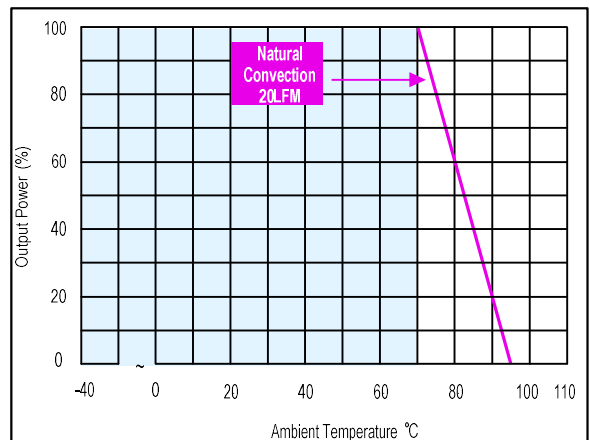
Figure 138: AYA01A48-L Derating Curve Vin = 48Vdc
