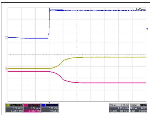
Figure 71: AYA01AA12-L Output Voltage Startup Characteristic by Vin Vin = 12Vdc Load: Io = ±0.3A Ch 3: Vin Ch 1: Vo1 Ch 2: Vo2
