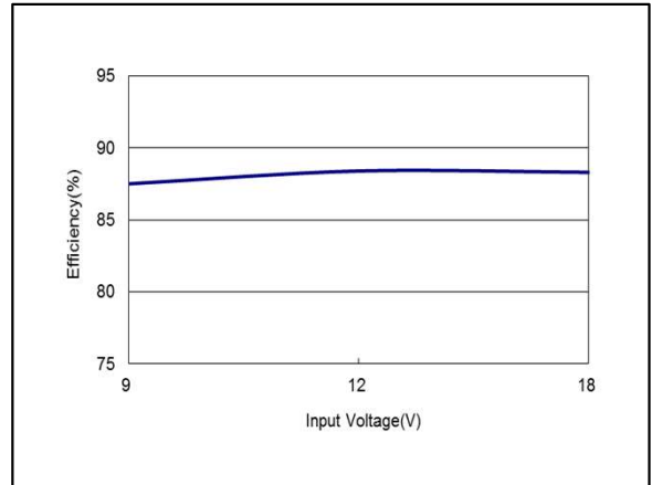
Figure 74: AYA01BB12-L Efficiency Versus Input Voltage Curve Vin = 9 to 18Vdc Load: Io = ±0.1A
