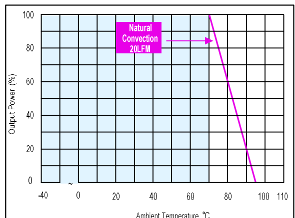
Figure 48: AYA01F12-L Derating Curve Vin = 12Vdc
