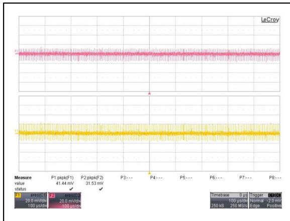
Figure 81: AYA01CC12-L Ripple and Noise Measurement Vin = 12Vdc Load: Io = ±0.1A Ch 1: Vo1 Ch 2: Vo2
