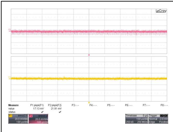
Figure 159: AYA01BB48-L Ripple and Noise Measurement Vin = 48Vdc Load: I_o = \pm 0.125A Ch 1: Vo
