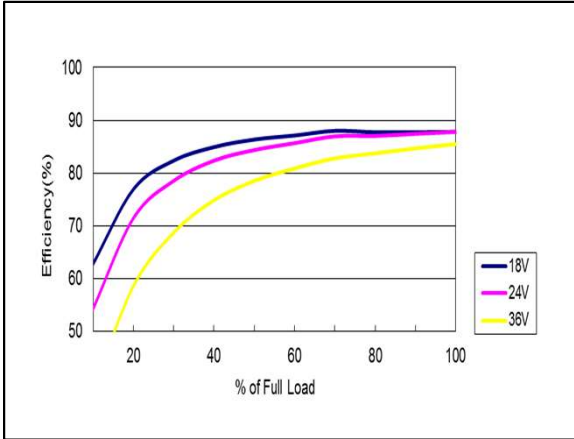
Figure 115: AYA01BB24-L Efficiency Versus Output Current Curve Vin = 18 to 36Vdc Load: Io = 0 to ±0.1A
