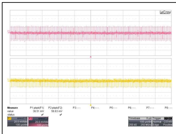
Figure 33: AYA01BB05-L Ripple and Noise Measurement Vin = 5Vdc Load: I_o = \pm 0.125A Ch 1: Vo1 Ch 2: Vo2
