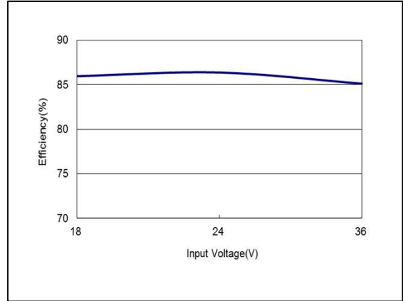
Figure 110: AYA01AA24-L Efficiency Versus Input Voltage Curve Vin = 18 to 36Vdc Load: Io = ±0.3A
