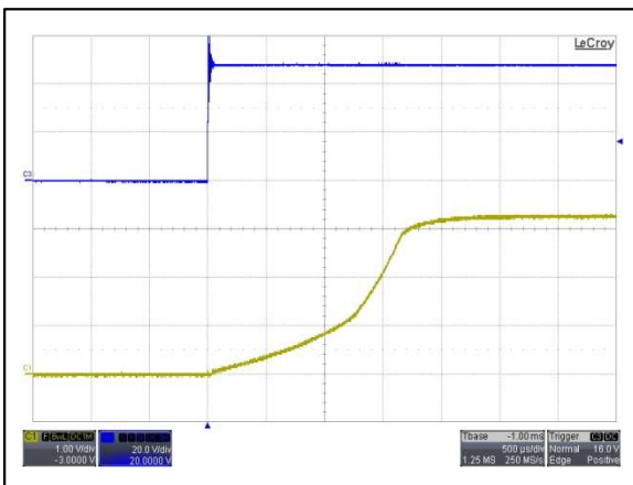
Figure 131: AYA01F48-L Output Voltage Startup Characteristic by Vin Vin = 48Vdc Load: Io = 0.6A Ch 3: Vin Ch 1: Vo
