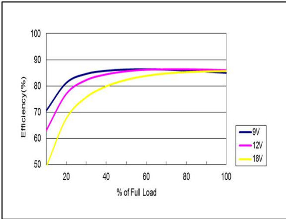
Figure 49: AYA01A12-L Efficiency Versus Output Current Curve Vin = 9 to 18Vdc Load: Io = 0 to 0.6A
