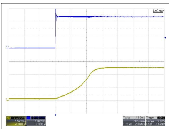
Figure 53: AYA01A12-L Output Voltage Startup Characteristic by Vin Vin = 12Vdc Load: Io = 0.6A Ch 3: Vin Ch 1: Vo
