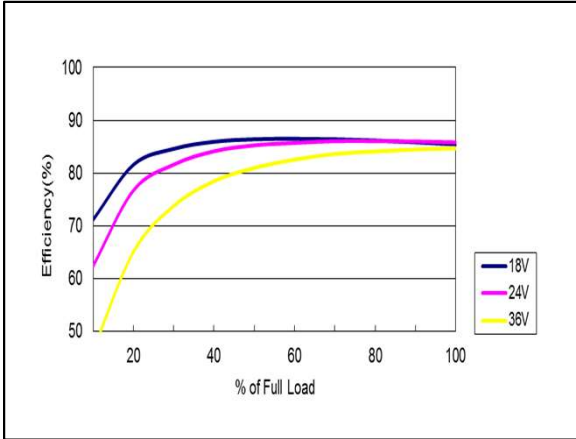
Figure 91: AYA01A24-L Efficiency Versus Output Current Curve Vin = 18 to 36Vdc Load: Io = 0 to 0.6A
