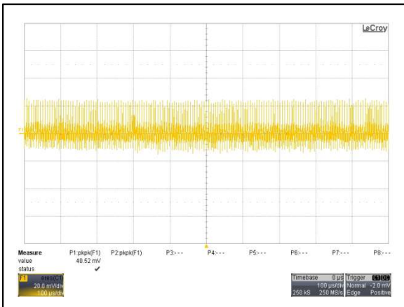
Figure 135: AYA01A48-L Ripple and Noise Measurement Vin = 48Vdc Load: Io = 0.6A Ch 1: Vo
