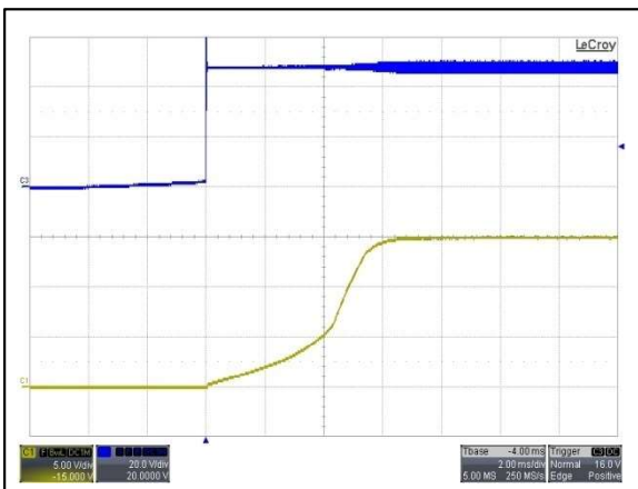
Figure 149: AYA01C48-L Output Voltage Startup Characteristic by Vin Vin = 48Vdc Load: Io = 0.2A Ch 3: Vin Ch 1: Vo
