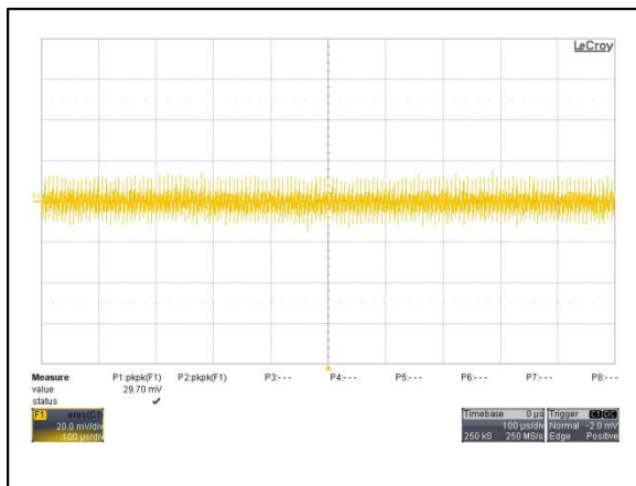
Figure 9: AYA01A05-L Ripple and Noise Measurement Vin = 5Vdc Load: Io = 0.6A Ch 1: Vo
