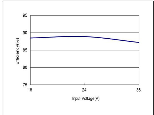
Figure 122: AYA01CC24-L Efficiency Versus Input Voltage Curve Vin = 18 to 36Vdc Load: Io = ±0.1A
