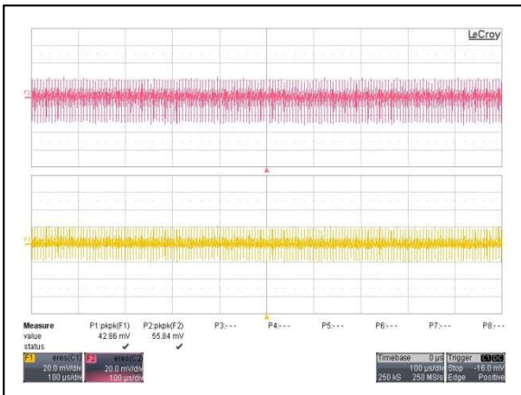
Figure 153: AYA01AA48-L Ripple and Noise Measurement Vin = 48Vdc Load: I_o = \pm 0.3A Ch 1: Vo
