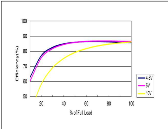
Figure 13: AYA01B05-L Efficiency Versus Output Current Curve Vin = 4.5 to 10Vdc Load: Io = 0 to 0.25A
