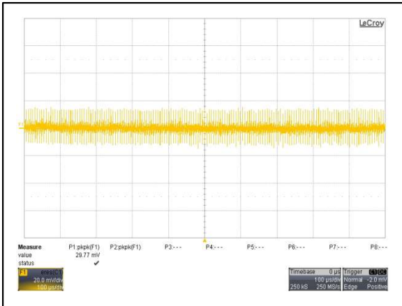
Figure 93: AYA01A24-L Ripple and Noise Measurement Vin = 24Vdc Load: Io = 0.6A Ch 1: Vo
