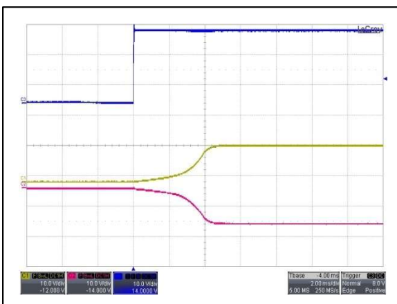
Figure 119: AYA01BB24-L Output Voltage Startup Characteristic by Vin Vin = 24Vdc Load: Io = ±0.1A Ch 3: Vin Ch 1: Vo1 Ch 2: Vo2
