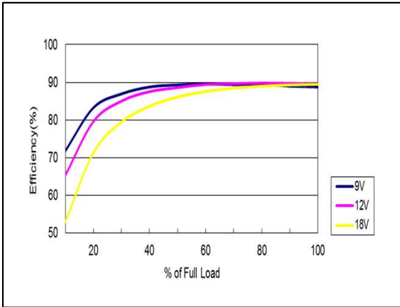
Figure 61: AYA01C12-L Efficiency Versus Output Current Curve Vin = 9 to 18Vdc Load: Io = 0 to 0.2A
