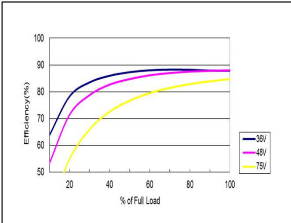
Figure 145: AYA01C48-L Efficiency Versus Output Current Curve Vin = 36 to 75Vdc Load: Io = 0 to 0.2A
