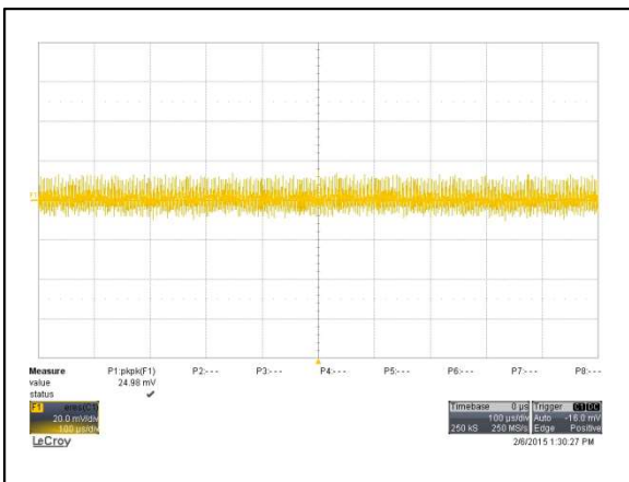
Figure 141: AYA01B48-L Ripple and Noise Measurement Vin = 48Vdc Load: Io = 0.25A Ch 1: Vo
