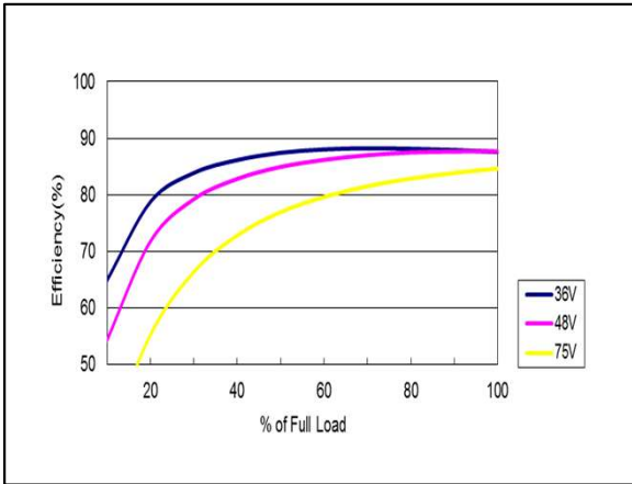
Figure 139: AYA01B48-L Efficiency Versus Output Current Curve Vin = 36 to 75Vdc Load: Io = 0 to 0.25A
