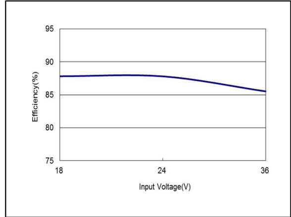
Figure 116: AYA01BB24-L Efficiency Versus Input Voltage Curve Vin = 18 to 36Vdc Load: Io = ±0.1A
