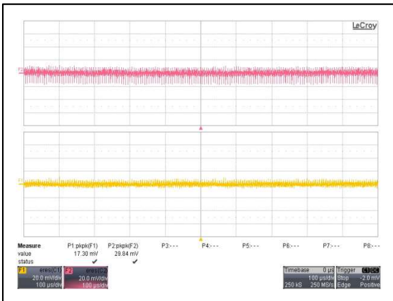
Figure 117: AYA01BB24-L Ripple and Noise Measurement Vin = 24Vdc Load: Io = ±0.1A Ch 1: Vo1 Ch 2: Vo2
