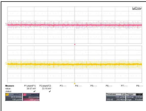
Figure 75: AYA01BB12-L Ripple and Noise Measurement Vin = 12Vdc Load: Io = ±0.1A Ch 1: Vo1 Ch 2: Vo2
