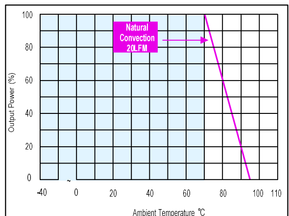
Figure 126: AYA01CC24-L Derating Curve Vin = 24Vdc
