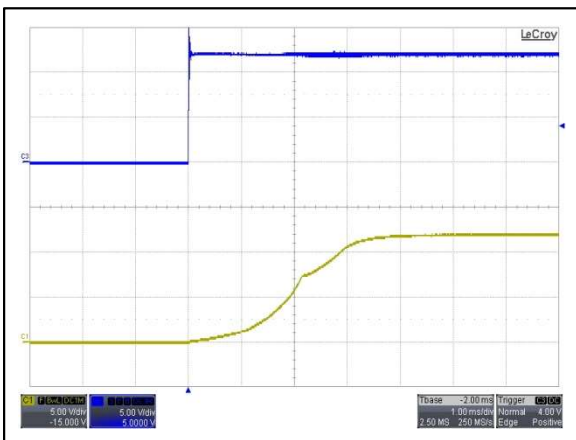
Figure 59: AYA01B12-L Output Voltage Startup Characteristic by Vin Vin = 12Vdc Load: Io = 0.25A Ch 3: Vin Ch 1: Vo
