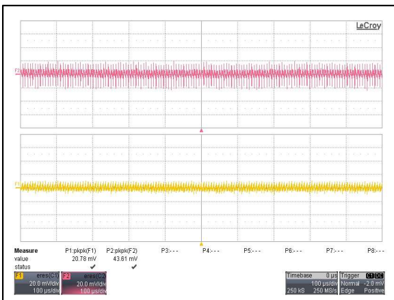
Figure 39: AYA01CC05-L Ripple and Noise Measurement Vin = 5Vdc Load: Io = ±0.1A Ch 1: Vo1 Ch 2: Vo2
