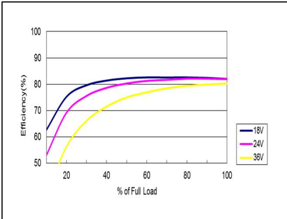
Figure 85: AYA01F24-L Efficiency Versus Output Current Curve Vin = 18 to 36Vdc Load: Io = 0 to 0.6A
