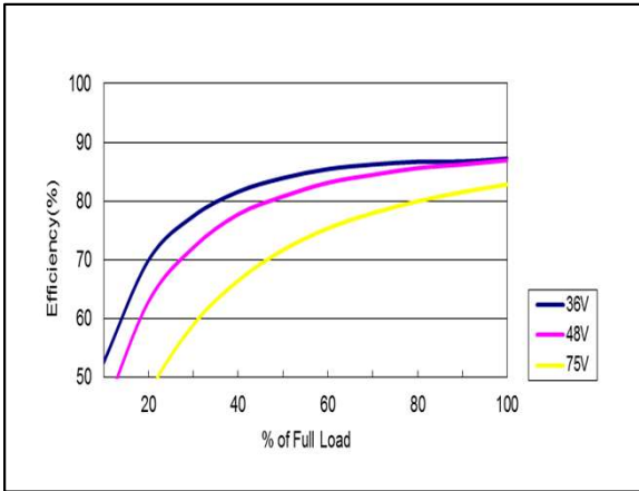
Figure 163: AYA01CC48-L Efficiency Versus Output Current Curve Vin = 36 to 75Vdc Load: I_o = 0 to \pm 0.1A
