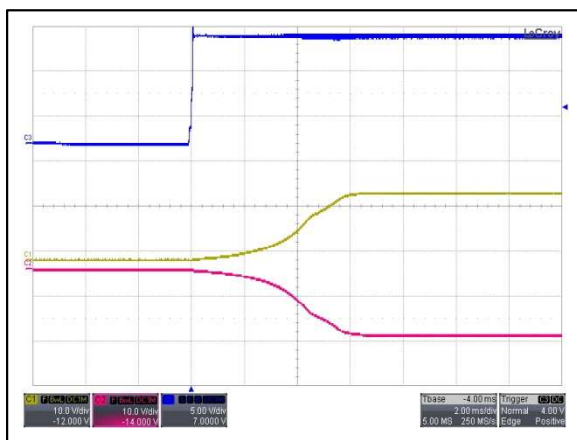
Figure 83: AYA01CC12-L Output Voltage Startup Characteristic by Vin Vin = 12Vdc Load: Io = ±0.1A Ch 3: Vin Ch 1: Vo1 Ch 2: Vo2
