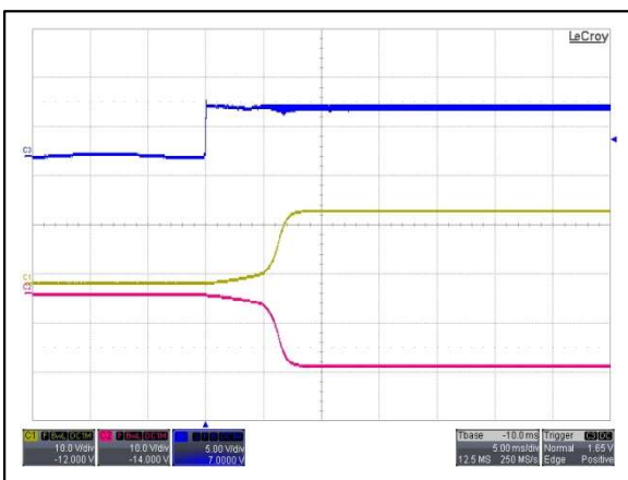
Figure 41: AYA01CC05-L Output Voltage Startup Characteristic by Vin Vin = 5Vdc Load: Io = ±0.1A Ch 3: Vin Ch 1: Vo1 Ch 2: Vo2
