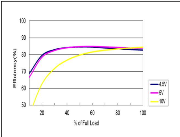
Figure 25: AYA01AA05-L Efficiency Versus Output Current Curve Vin = 4.5 to 10Vdc Load: lo = 0 to ±0.3A
