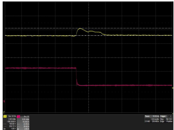
Figure 24: iHP24H3A-SA-00 Transient Response - V_o Deviation 100% to 50% load change, 0.5A/\mu S slew rate Ch 1: V_o Ch 2: I_o
