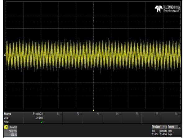
Figure 22: iHP24H3A-SA-00 Ripple and Noise Measurement Load: I_o = 15A Ch 1: V_o
