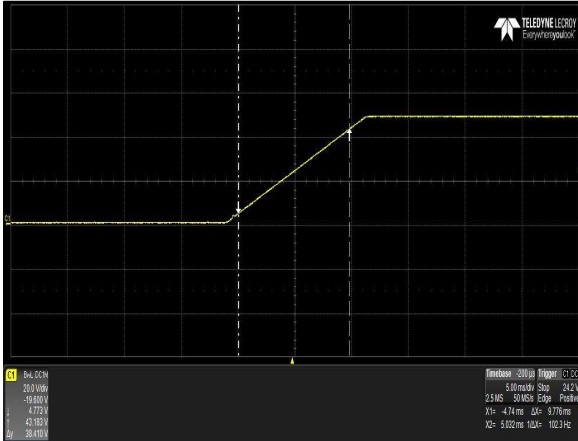
Figure 39: iHP24H3A-SW-00 Output Voltage Startup Characteristic Load: I_o = 62.5A Ch 1: V_o
