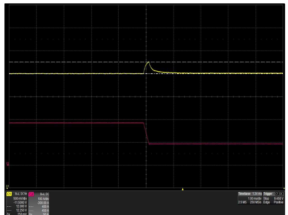
Figure 60: iHP24H3A-SL-00 Transient Response - V_o Deviation 100% to 50% load change, 0.5A/\mu S slew rate Ch 1: V_o Ch 2: I_o
