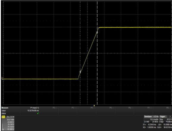
Figure 33: iHP24H3A-S8-00 Output Voltage Startup Characteristic Load: I_o = 37.5A Ch 1: V_o
