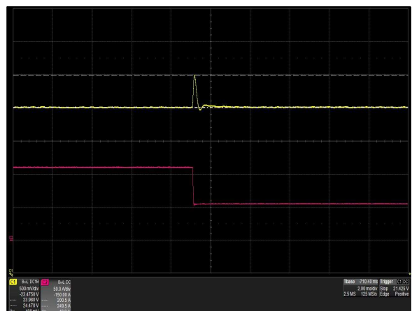
Figure 54: iHP24H3A-SQ-00 Transient Response - V_o Deviation 100% to 50% load change, 0.5A/\mu S slew rate Ch 1: V_o Ch 2: I_o
