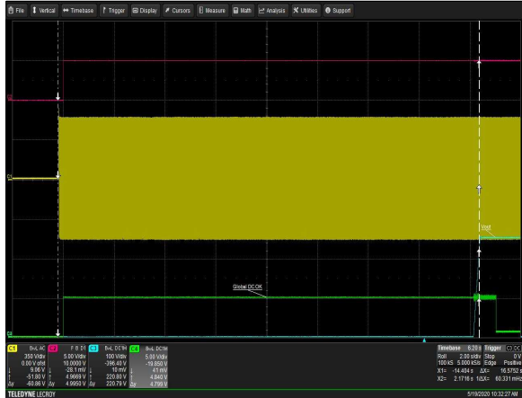
Figure 1: iHP24H3A-S2-00 Turn-on delay via AC mains Vin = 380Vac Load: I_O = 12A I_{SB} = 1A Ch 1: AC Mains Ch 2: V_{SB} Ch 3: V_O Ch 4: Global DCOK
