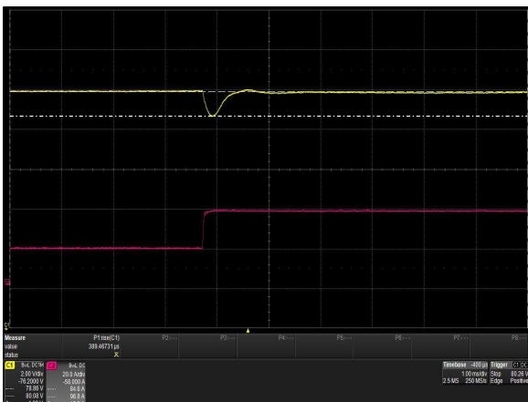
Figure 35: iHP24H3A-S8-00 Transient Response - V_o Deviation 50% to 100% load change, 0.5A/\mu S slew rate Ch 1: V_o Ch 2: I_o
