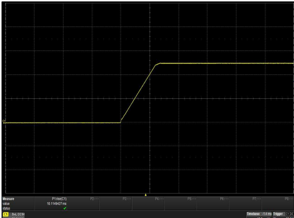
Figure 27: iHP24H3A-S1-00 Output Voltage Startup Characteristic Load: I_o = 12A Ch 1: V_o
