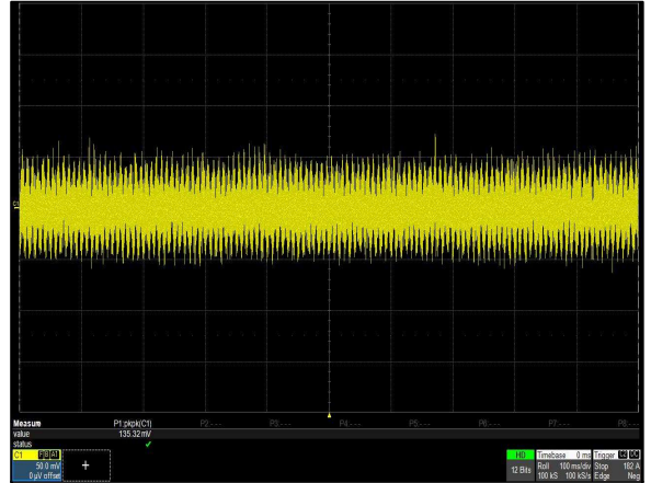
Figure 64: iHP12L1A-TW-00 Ripple and Noise Measurement Load: I_o = 240A Ch 1: V_o
