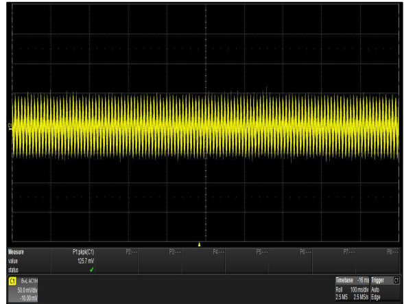
Figure 46: iHP24H3A-ST-00 Ripple and Noise Measurement Load: I_o = 90A Ch 1: V_o
