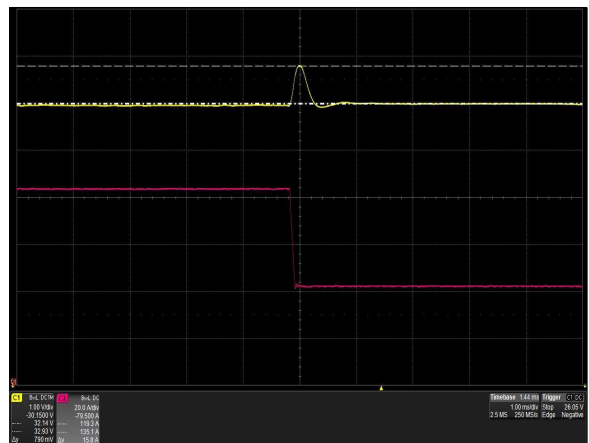
Figure 48: iHP24H3A-ST-00 Transient Response - V_o Deviation 100% to 50% load change, 0.5A/\mu S slew rate Ch 1: V_o Ch 2: I_o
