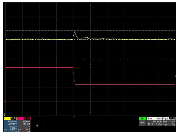
Figure 66: iHP12L1A-TW-00 Transient Response - V_o Deviation 100% to 50% load change, 0.5A/\mu S slew rate Ch 1: V_o Ch 2: I_o
