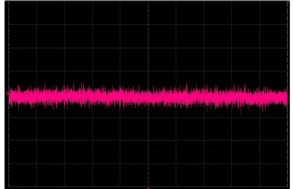
Figure 26: iHP24H3A-SA-00 Ripple and Noise Measurement Load: R = 13.3 ohm Ch 2: I_o
