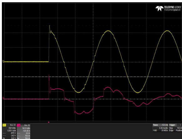
Figure 5: iHP24H3A-S2-00 Start up Inrush Current Vin = 528Vac Load: I_O = 0A Turn On Phase = 90° Ch 1: V_{IN} Ch 2: I_{IN}
