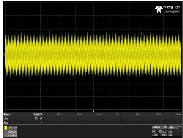
Figure 52: iHP24H3A-SQ-00 Ripple and Noise Measurement Load: I_o = 120A Ch 1: V_o
