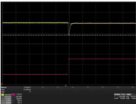
Figure 41: iHP24H3A-SW-00 Transient Response - V_o Deviation 50% to 100% load change, 0.5A/ \mu S slew rate Ch 1: V_o Ch 2: I_o
