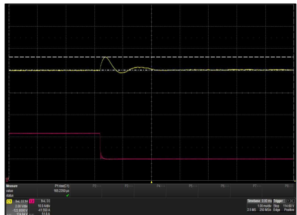
Figure 30: iHP24H3A-S1-00 Transient Response - V_o Deviation 100% to 50% load change, 0.5A/\mu S slew rate Ch 1: V_o Ch 2: I_o
