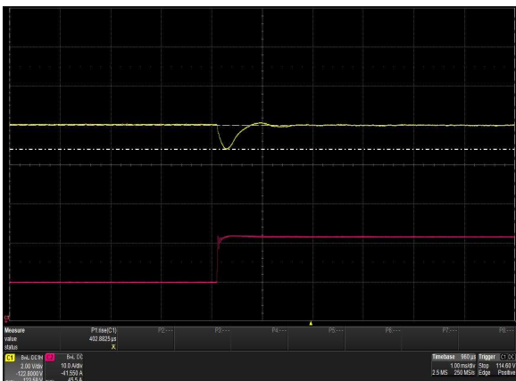
Figure 29: iHP24H3A-S1-00 Transient Response - V_o Deviation 50% to 100% load change, 0.5A/\mu S slew rate Ch 1: V_o Ch 2: I_o
